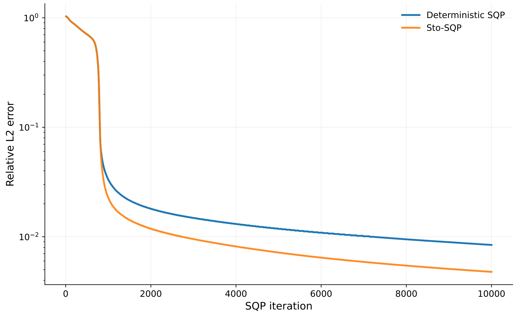
Allen-Cahn equation: relative L2 error
